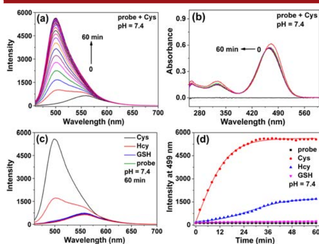
Figure 1. (a) Time-dependent fluorescence emission spectra of 1 (30 μM) in the presence of 10 equiv of Cys in Hepes buffer/DMSO (1:1, v/v, pH 7.4) at 25 °C. (b) Corresponding time-dependent UV-vis spectra of 1 (30 μM) in the presence of 10 equiv of Cys in Hepes buffer/DMSO (1:1, v/v, pH 7.4) at 25 °C. (c) Fluorescence emission spectra of 1 (30 μM) upon addition of 10 equiv of Cys, Hcy, GSH, Ala, Asn, Arg, Asp, Gln, Glu, Gly, His, Ile, Leu, Lys, Met, Phe, Pro, Ser, Thr, Trp, Tyr, and Val in Hepes buffer/DMSO (1:1, v/v, pH 7.4) at 25 °C. (d) Time-dependent fluorescence emission intensity changes of 1 toward 10 equiv of biothiols at 499 nm (λ ex = 447 nm, slit: 5 nm/5 nm).
