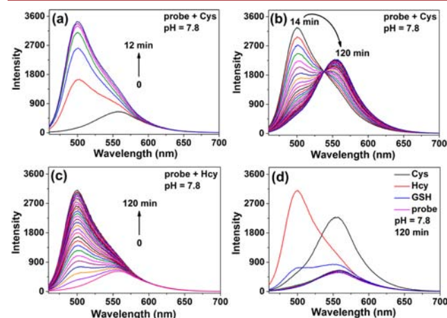
Figure 2. (a, b) Time-dependent fluorescence emission spectra of 1 (30 μM) in the presence of 10 equiv of Cys in Hepes buffer/DMSO (1:1, v/v, pH 7.8) at 25 °C. (c) Time-dependent fluorescence emission spectra of 1 (30 μM) in the presence of 10 equiv of Hcy in Hepes buffer/DMSO (1:1, v/v, pH 7.8) at 25 °C. (d) Fluorescence spectra of 1 (30 μM) upon addition of 10 equiv of Cys, Hcy, GSH, Ala, Asn, Arg, Asp, Gln, Glu, Gly, His, Ile, Leu, Lys, Met, Phe, Pro, Ser, Thr, Trp, Tyr, and Val in Hepes buffer/DMSO (1:1, v/v, pH 7.8) at 25 °C. (λ ex = 447 nm, slit: 5 nm/5 nm).
